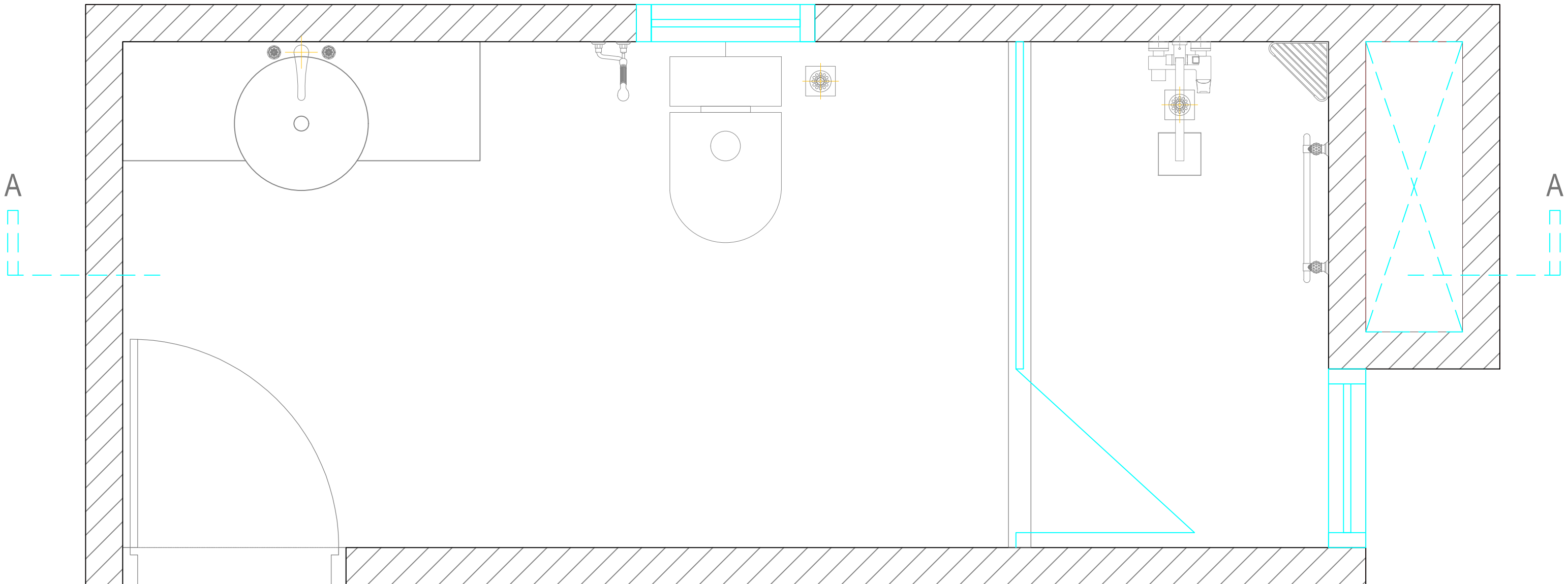
MASTER BEDROOM TOILET LAYOUT SCALE: NOT TO SCALE
