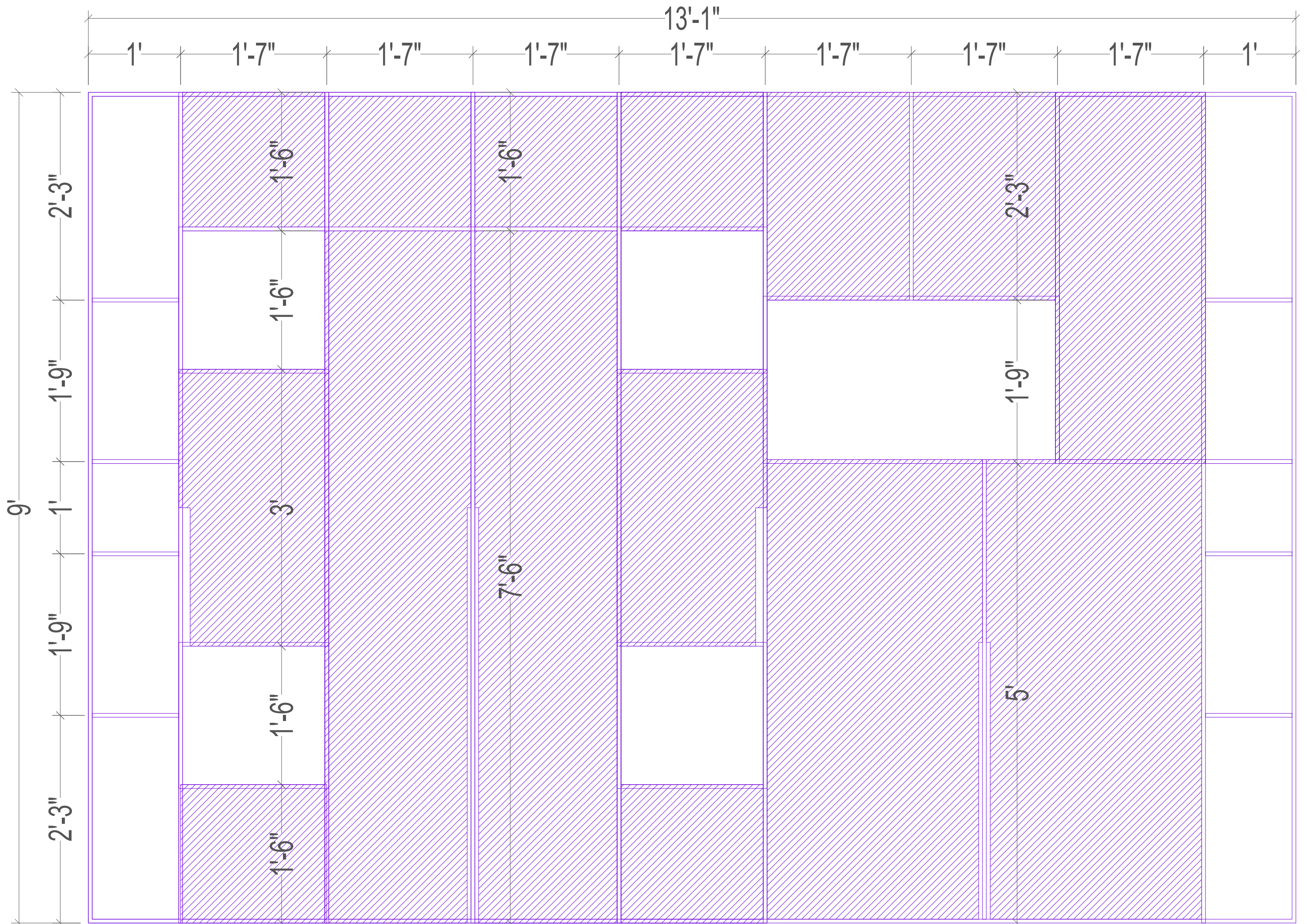
Child Bedroom-Cabinet design
